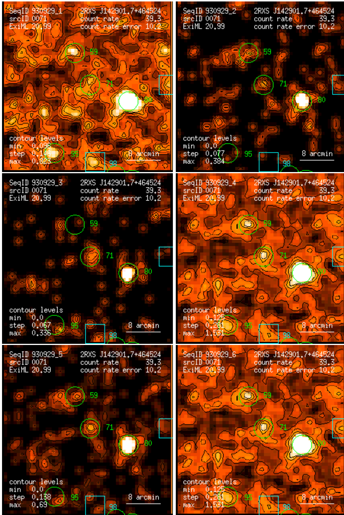
Figure 71: RASS 930929: detection 0071: band rate images, Gaussian filter: (1) PSPC channels 11 – 41, (2) 52 – 90, (3) 91 – 201, (4) 11 – 235, (5) 52 – 201, (6) 11 – 201. Broad band rates in counts/ks. Band rate contour levels in counts/ks/arcmin 2 .
