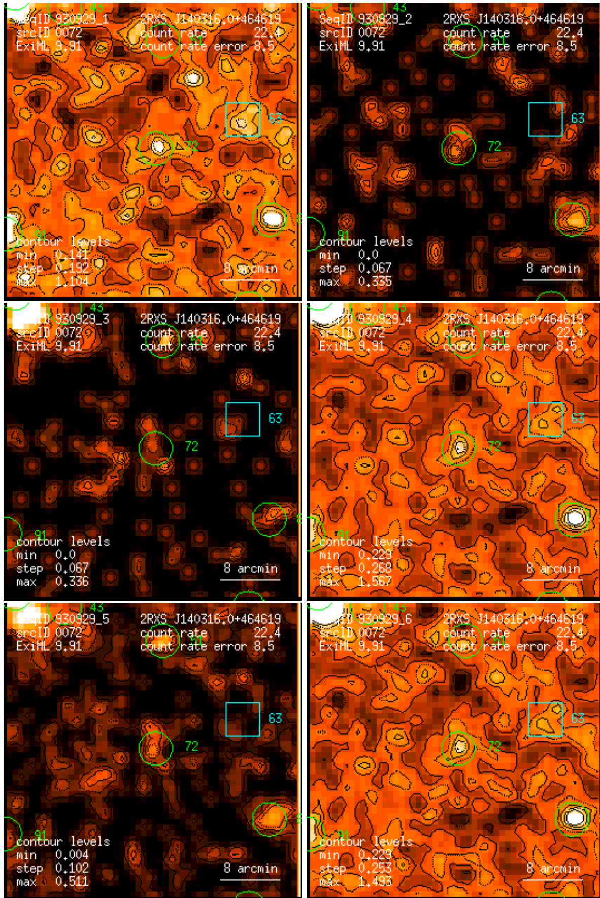
Figure 72: RASS 930929: detection 0072: band rate images, Gaussian filter: (1) PSPC channels 11 – 41, (2) 52 – 90, (3) 91 – 201, (4) 11 – 235, (5) 52 – 201, (6) 11 – 201. Broad band rates in counts/ks. Band rate contour levels in counts/ks/arcmin 2 .
