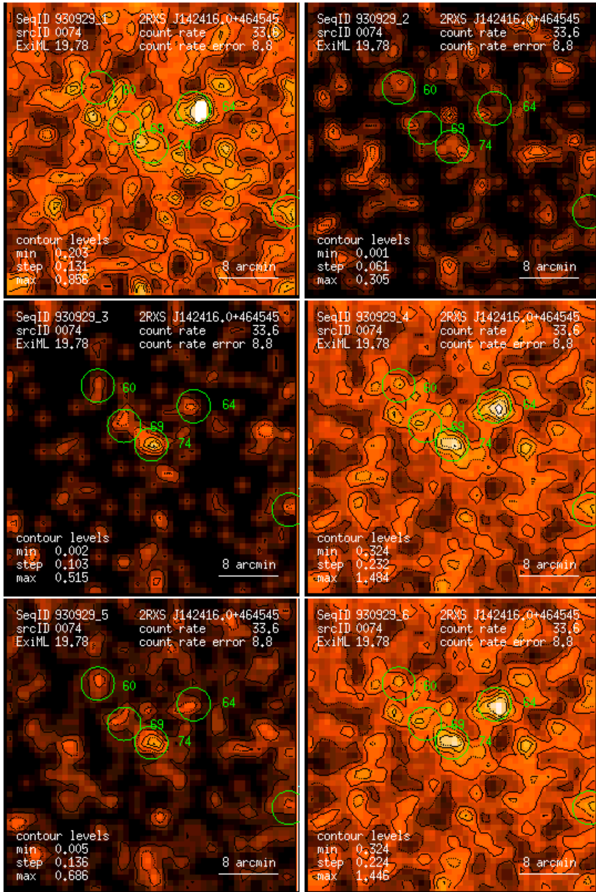
Figure 74: RASS 930929: detection 0074: band rate images, Gaussian filter: (1) PSPC channels 11 – 41, (2) 52 – 90, (3) 91 – 201, (4) 11 – 235, (5) 52 – 201, (6) 11 – 201. Broad band rates in counts/ks. Band rate contour levels in counts/ks/arcmin 2 .
