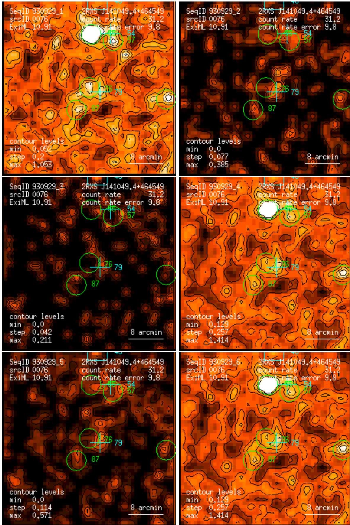
Figure 76: RASS 930929: detection 0076: band rate images, Gaussian filter: (1) PSPC channels 11 – 41, (2) 52 – 90, (3) 91 – 201, (4) 11 – 235, (5) 52 – 201, (6) 11 – 201. Broad band rates in counts/ks. Band rate contour levels in counts/ks/arcmin 2 .
