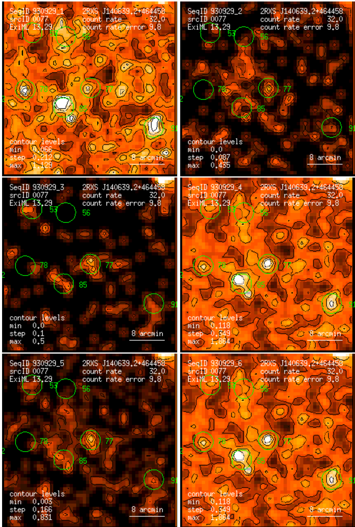
Figure 77: RASS 930929: detection 0077: band rate images, Gaussian filter: (1) PSPC channels 11 – 41, (2) 52 – 90, (3) 91 – 201, (4) 11 – 235, (5) 52 – 201, (6) 11 – 201. Broad band rates in counts/ks. Band rate contour levels in counts/ks/arcmin 2 .
