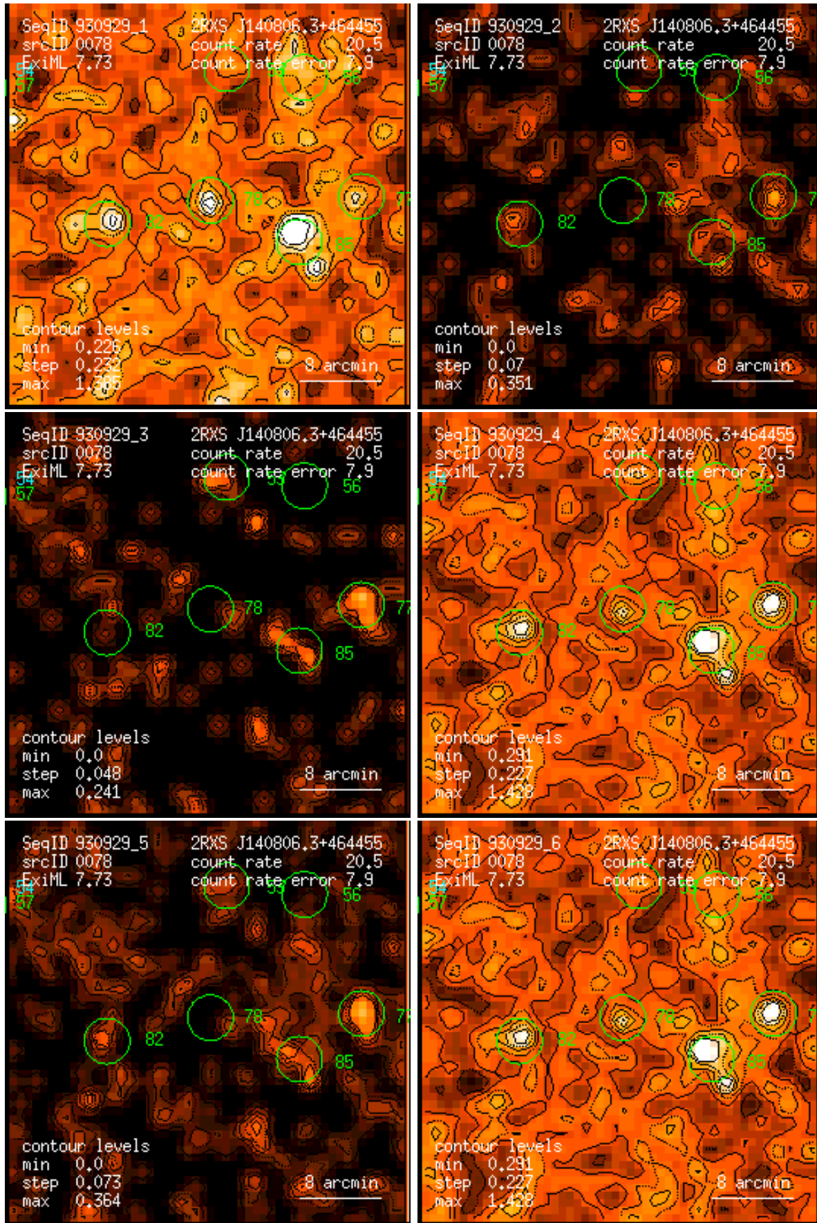
Figure 78: RASS 930929: detection 0078: band rate images, Gaussian filter: (1) PSPC channels 11 – 41, (2) 52 – 90, (3) 91 – 201, (4) 11 – 235, (5) 52 – 201, (6) 11 – 201. Broad band rates in counts/ks. Band rate contour levels in counts/ks/arcmin 2 .
