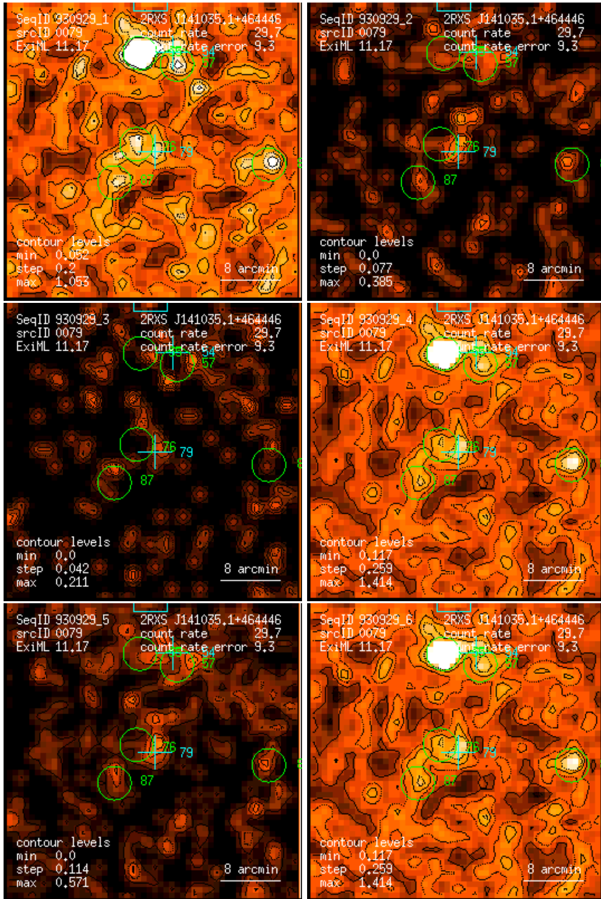
Figure 79: RASS 930929: detection 0079: band rate images, Gaussian filter: (1) PSPC channels 11 – 41, (2) 52 – 90, (3) 91 – 201, (4) 11 – 235, (5) 52 – 201, (6) 11 – 201. Broad band rates in counts/ks. Band rate contour levels in counts/ks/arcmin 2 .
