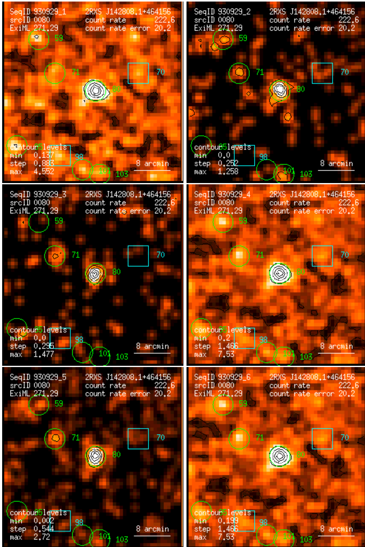
Figure 80: RASS 930929: detection 0080: band rate images, Gaussian filter: (1) PSPC channels 11 – 41, (2) 52 – 90, (3) 91 – 201, (4) 11 – 235, (5) 52 – 201, (6) 11 – 201. Broad band rates in counts/ks. Band rate contour levels in counts/ks/arcmin 2 .
