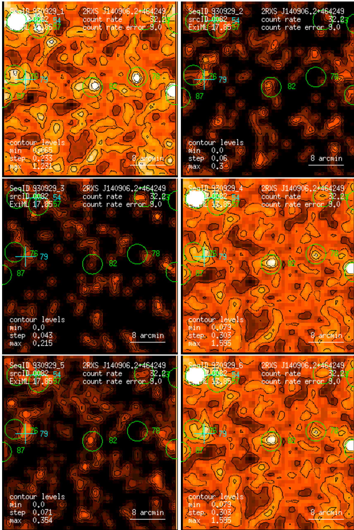
Figure 82: RASS 930929: detection 0082: band rate images, Gaussian filter: (1) PSPC channels 11 – 41, (2) 52 – 90, (3) 91 – 201, (4) 11 – 235, (5) 52 – 201, (6) 11 – 201. Broad band rates in counts/ks. Band rate contour levels in counts/ks/arcmin 2 .
