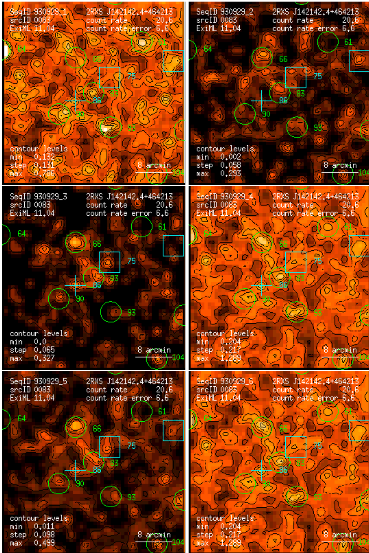
Figure 83: RASS 930929: detection 0083: band rate images, Gaussian filter: (1) PSPC channels 11 – 41, (2) 52 – 90, (3) 91 – 201, (4) 11 – 235, (5) 52 – 201, (6) 11 – 201. Broad band rates in counts/ks. Band rate contour levels in counts/ks/arcmin 2 .
