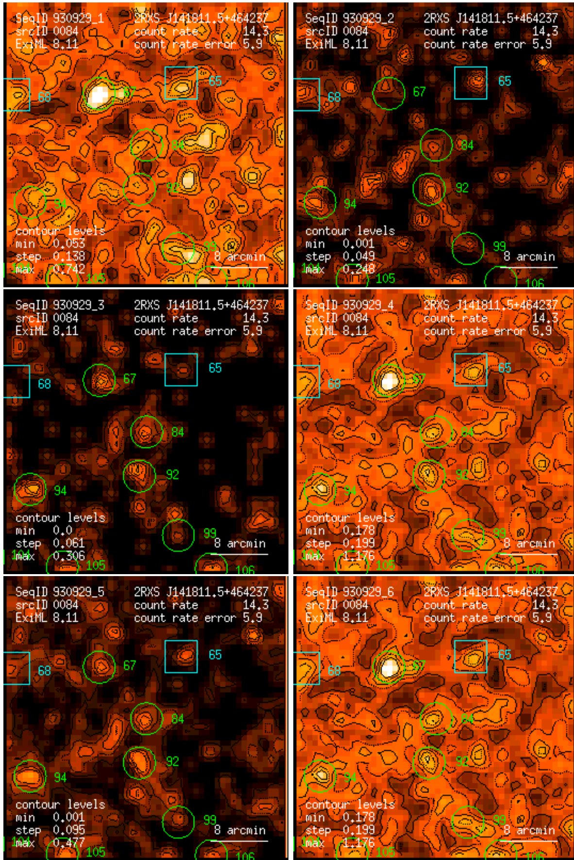
Figure 84: RASS 930929: detection 0084: band rate images, Gaussian filter: (1) PSPC channels 11 – 41, (2) 52 – 90, (3) 91 – 201, (4) 11 – 235, (5) 52 – 201, (6) 11 – 201. Broad band rates in counts/ks. Band rate contour levels in counts/ks/arcmin 2 .
