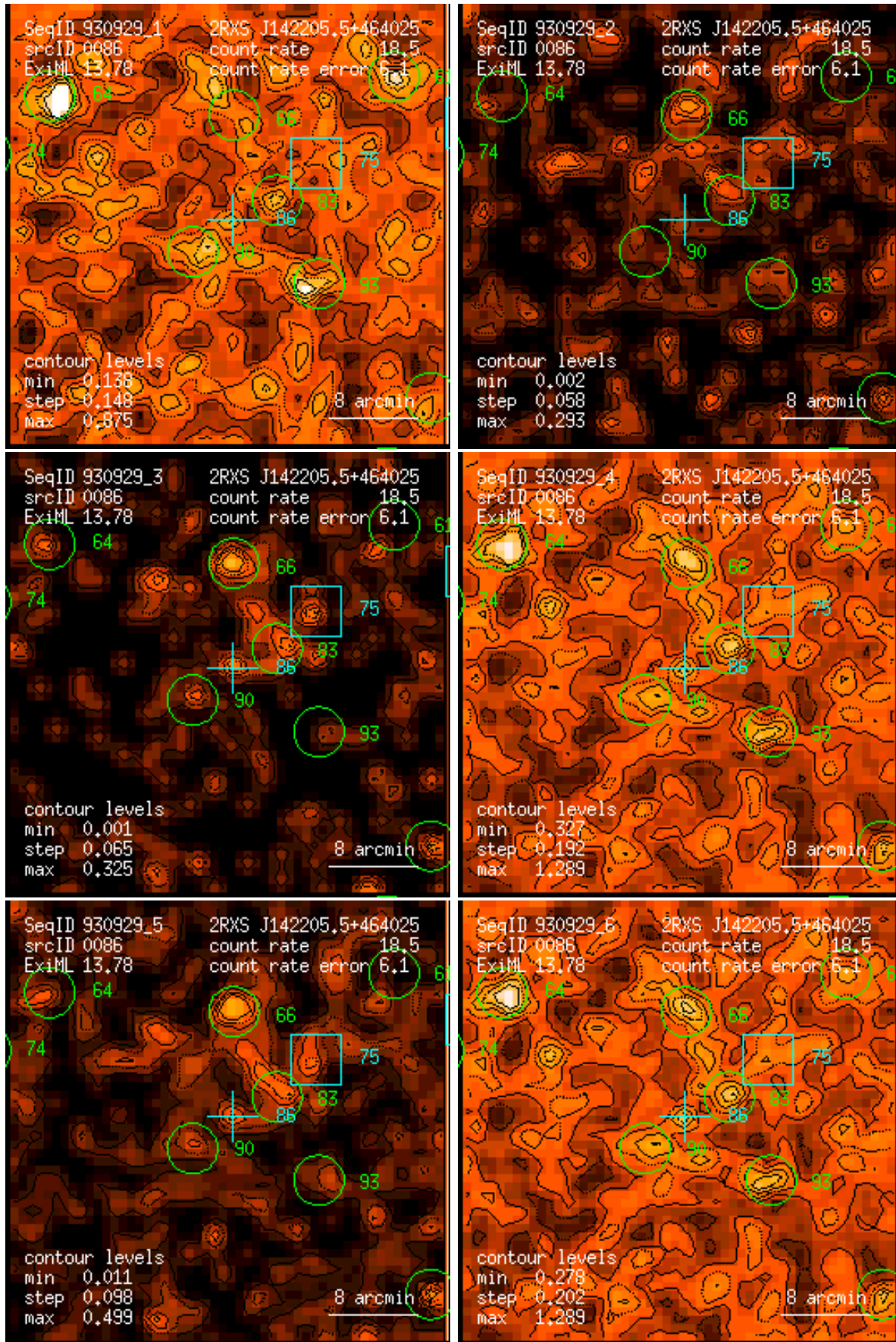
Figure 86: RASS 930929: detection 0086: band rate images, Gaussian filter: (1) PSPC channels 11 – 41, (2) 52 – 90, (3) 91 – 201, (4) 11 – 235, (5) 52 – 201, (6) 11 – 201. Broad band rates in counts/ks. Band rate contour levels in counts/ks/arcmin 2 .
