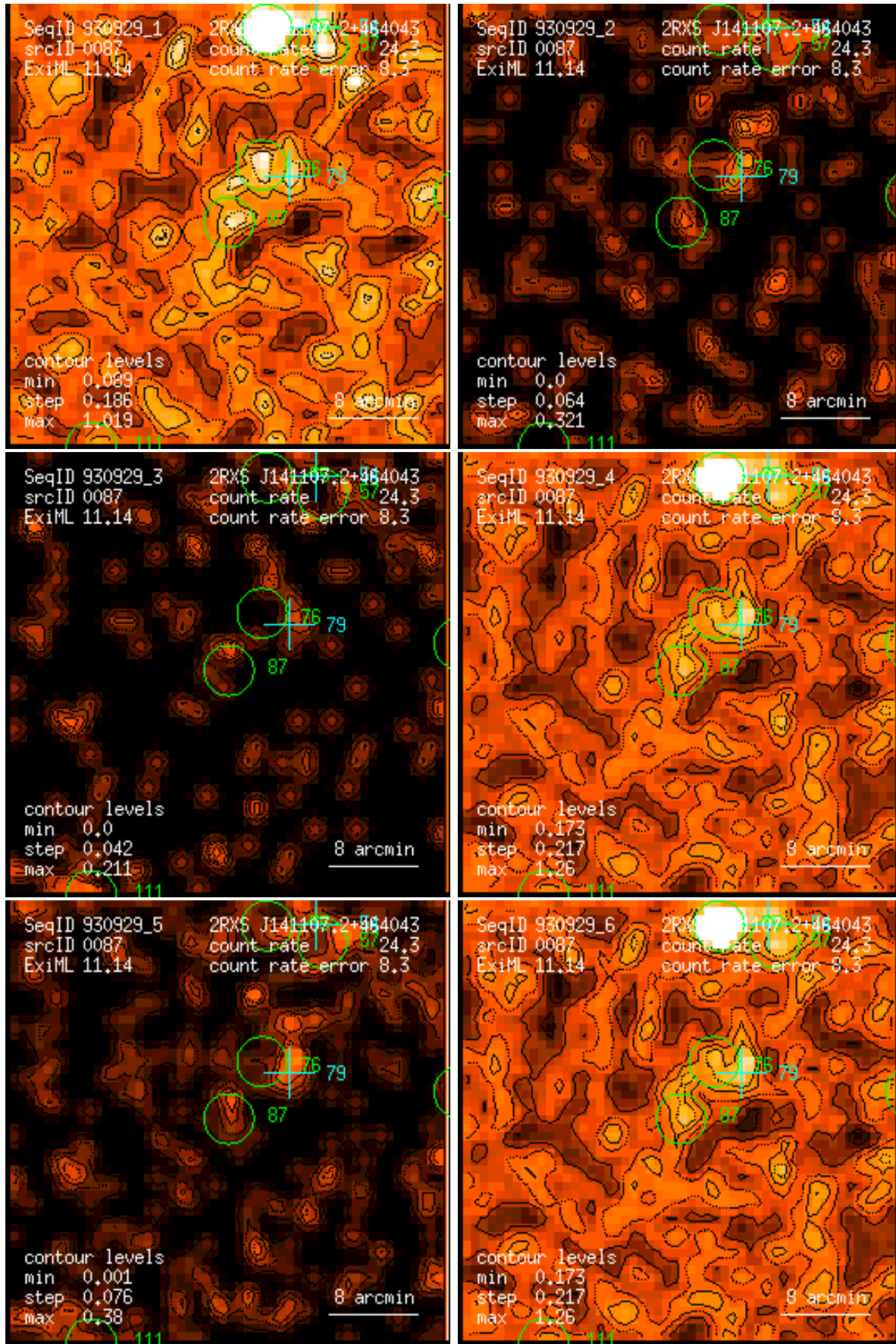
Figure 87: RASS 930929: detection 0087: band rate images, Gaussian filter: (1) PSPC channels 11 – 41, (2) 52 – 90, (3) 91 – 201, (4) 11 – 235, (5) 52 – 201, (6) 11 – 201. Broad band rates in counts/ks. Band rate contour levels in counts/ks/arcmin 2 .
