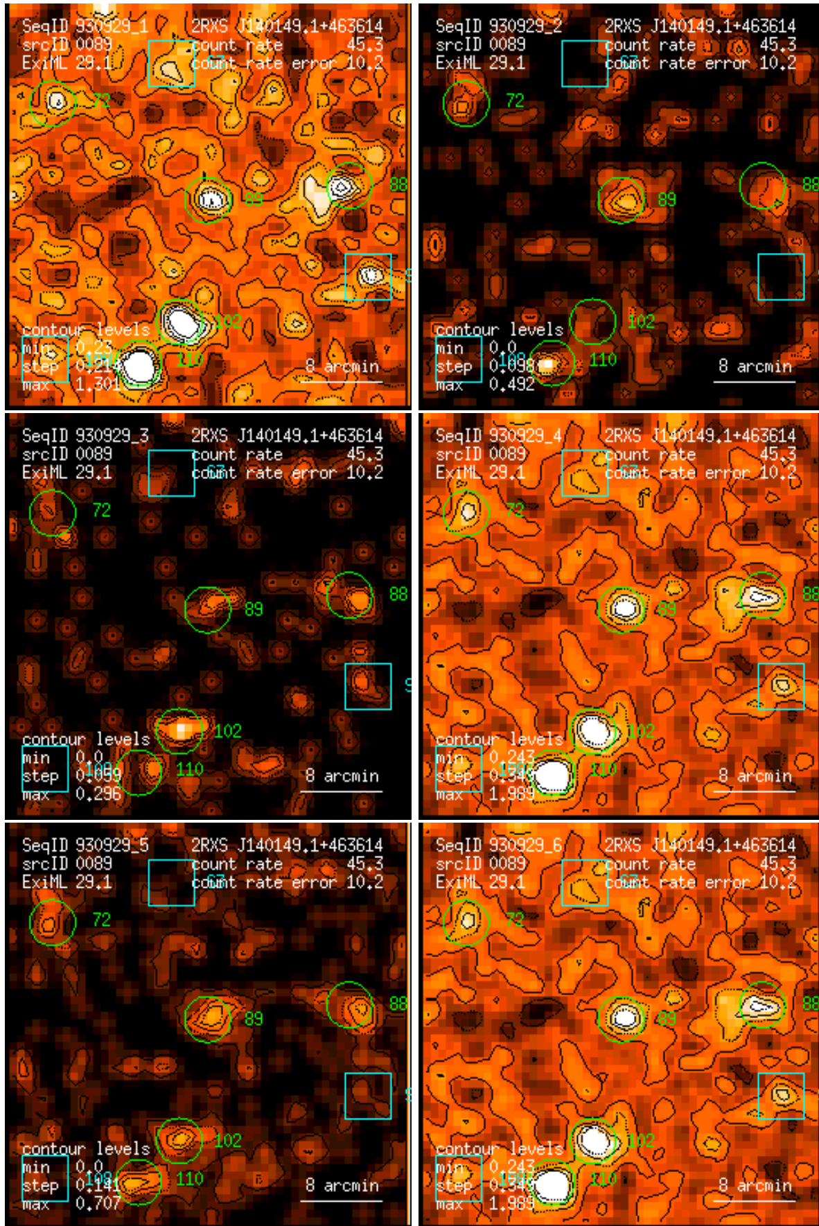
Figure 89: RASS 930929: detection 0089: band rate images, Gaussian filter: (1) PSPC channels 11 – 41, (2) 52 – 90, (3) 91 – 201, (4) 11 – 235, (5) 52 – 201, (6) 11 – 201. Broad band rates in counts/ks. Band rate contour levels in counts/ks/arcmin 2 .
