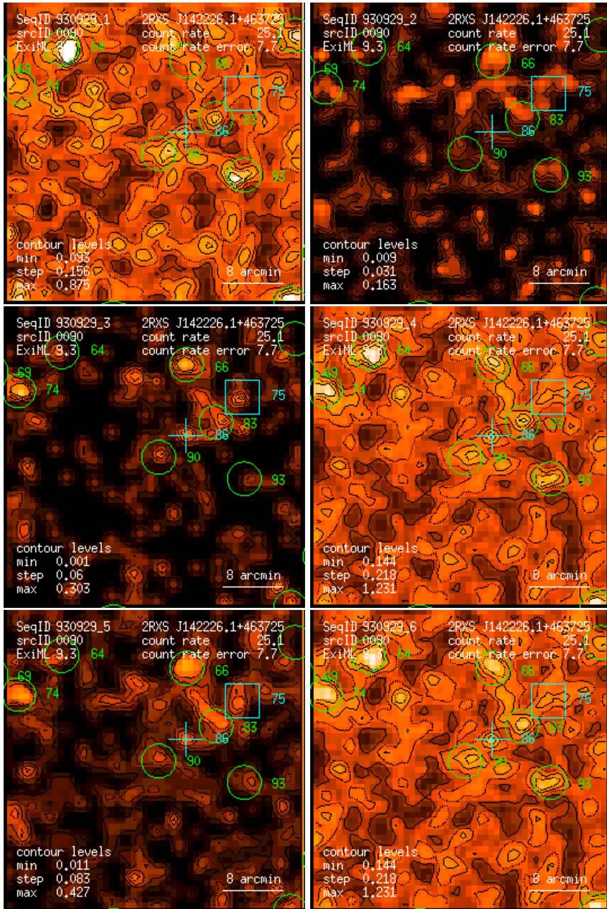
Figure 90: RASS 930929: detection 0090: band rate images, Gaussian filter: (1) PSPC channels 11 – 41, (2) 52 – 90, (3) 91 – 201, (4) 11 – 235, (5) 52 – 201, (6) 11 – 201. Broad band rates in counts/ks. Band rate contour levels in counts/ks/arcmin 2 .
