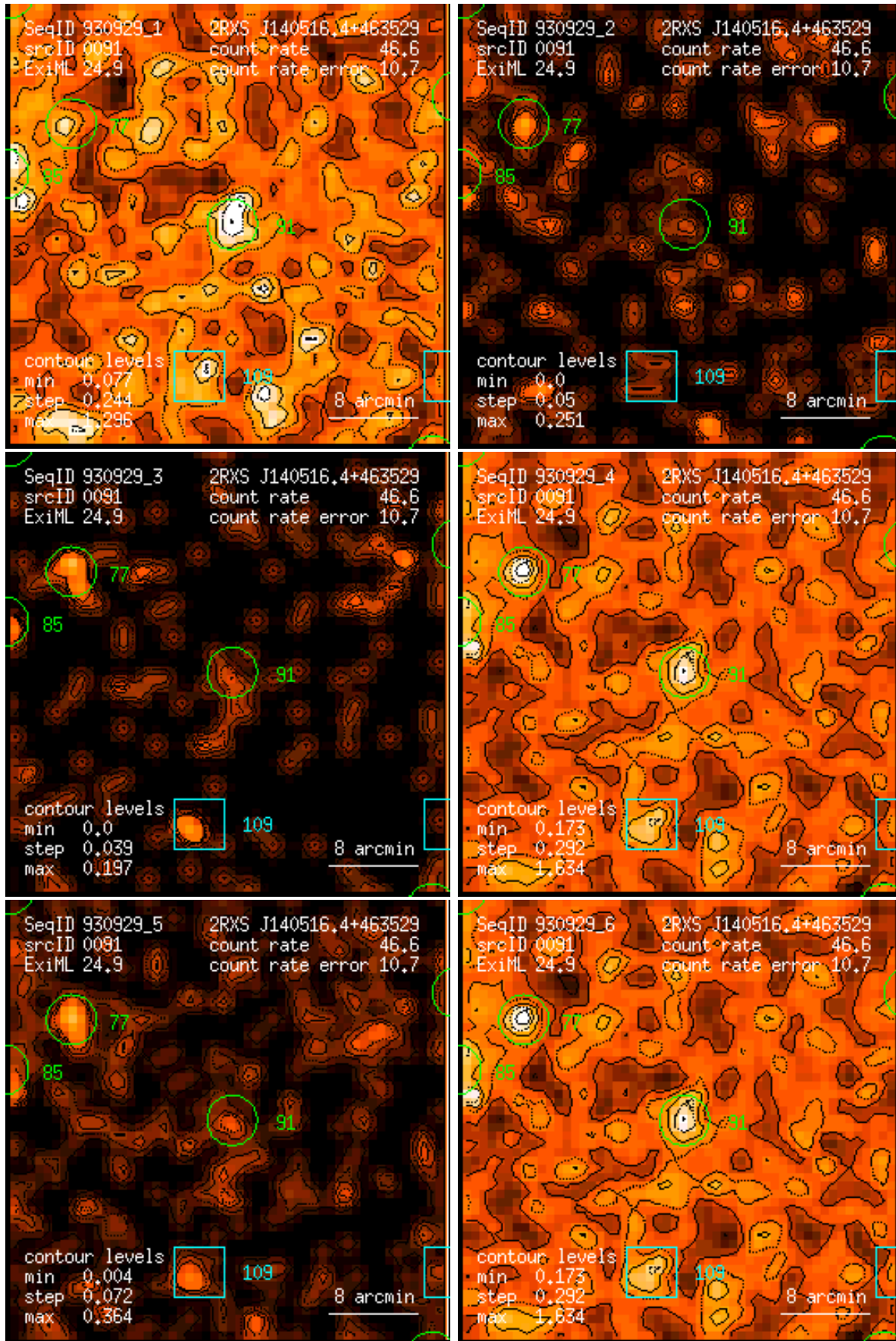
Figure 91: RASS 930929: detection 0091: band rate images, Gaussian filter: (1) PSPC channels 11 – 41, (2) 52 – 90, (3) 91 – 201, (4) 11 – 235, (5) 52 – 201, (6) 11 – 201. Broad band rates in counts/ks. Band rate contour levels in counts/ks/arcmin 2 .
