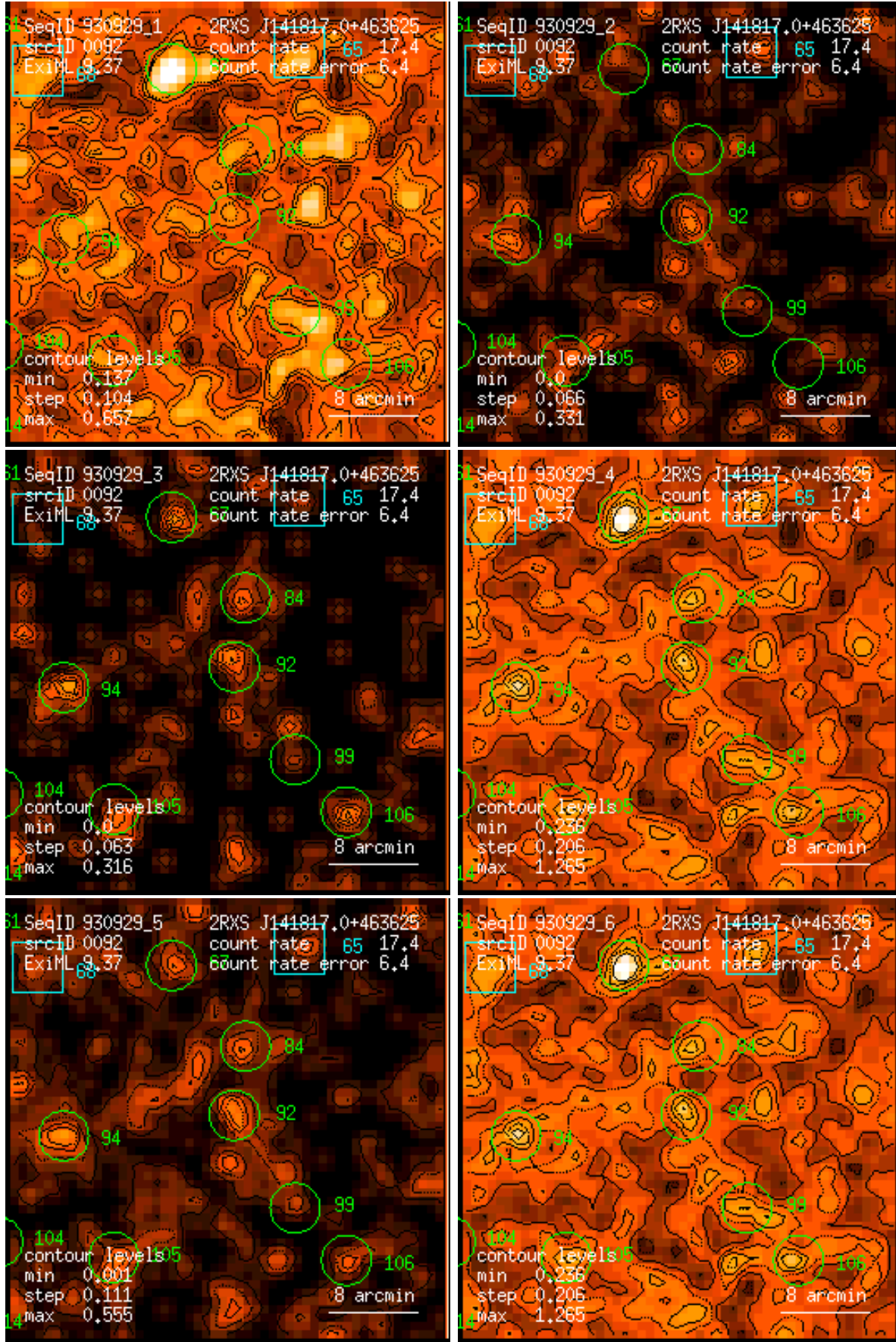
Figure 92: RASS 930929: detection 0092: band rate images, Gaussian filter: (1) PSPC channels 11 – 41, (2) 52 – 90, (3) 91 – 201, (4) 11 – 235, (5) 52 – 201, (6) 11 – 201. Broad band rates in counts/ks. Band rate contour levels in counts/ks/arcmin 2 .
