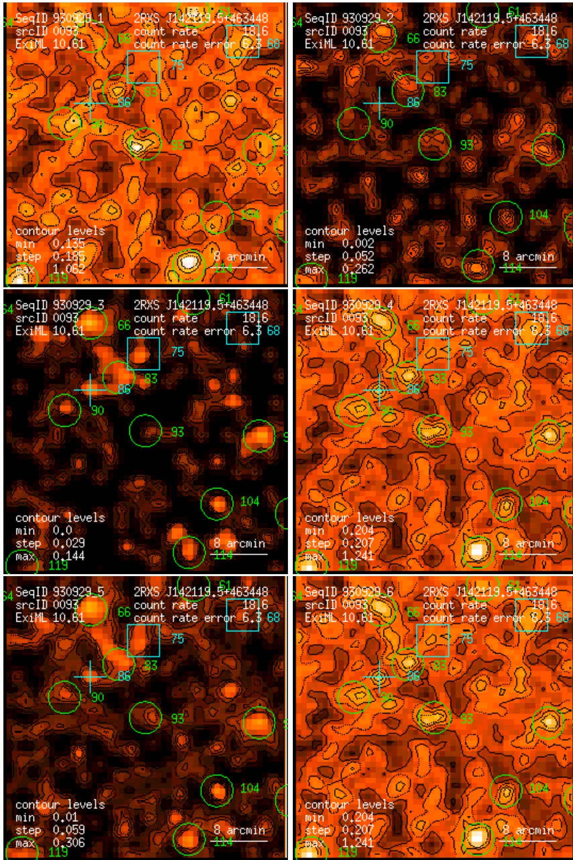
Figure 93: RASS 930929: detection 0093: band rate images, Gaussian filter: (1) PSPC channels 11 – 41, (2) 52 – 90, (3) 91 – 201, (4) 11 – 235, (5) 52 – 201, (6) 11 – 201. Broad band rates in counts/ks. Band rate contour levels in counts/ks/arcmin 2 .
