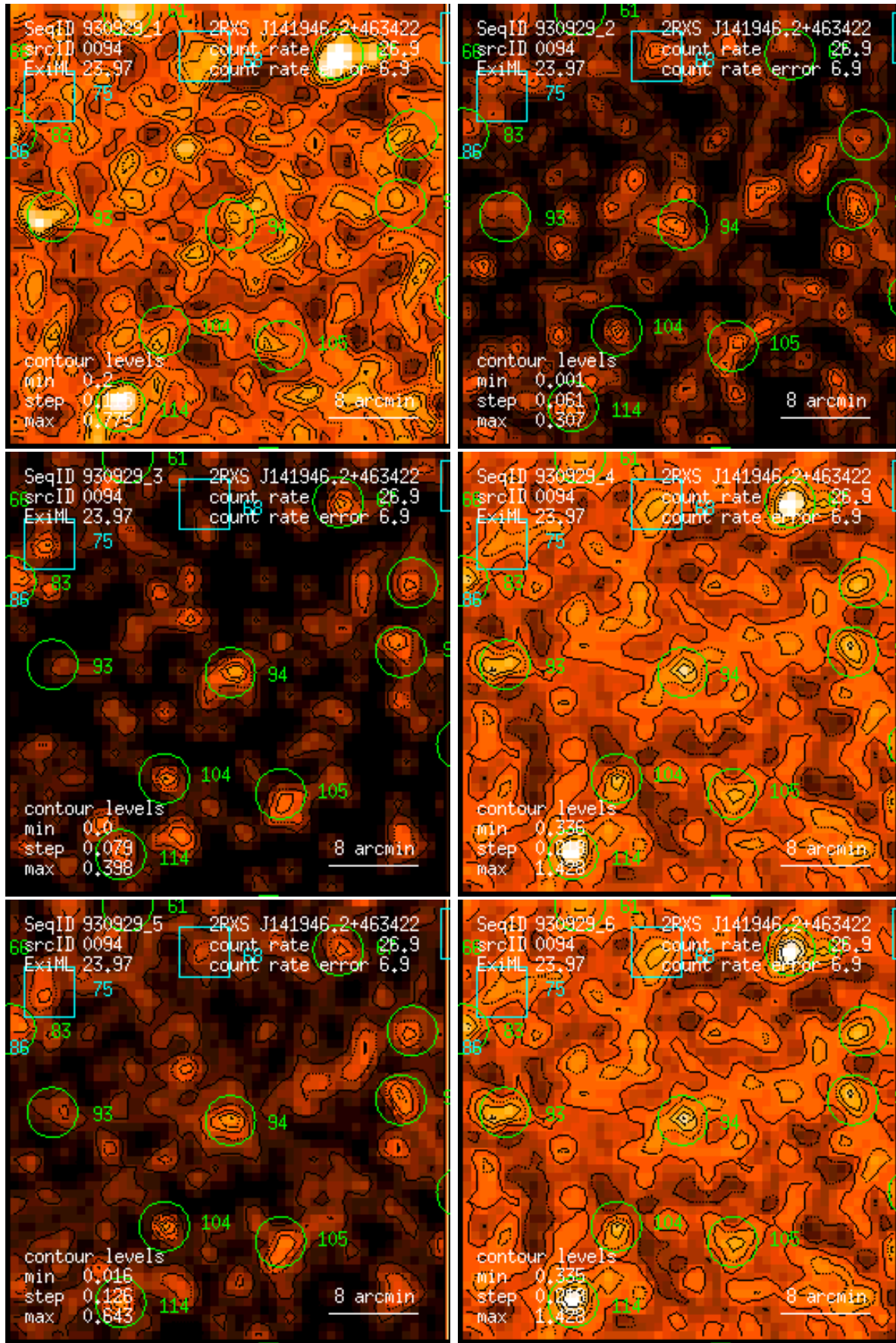
Figure 94: RASS 930929: detection 0094: band rate images, Gaussian filter: (1) PSPC channels 11 – 41, (2) 52 – 90, (3) 91 – 201, (4) 11 – 235, (5) 52 – 201, (6) 11 – 201. Broad band rates in counts/ks. Band rate contour levels in counts/ks/arcmin 2 .
