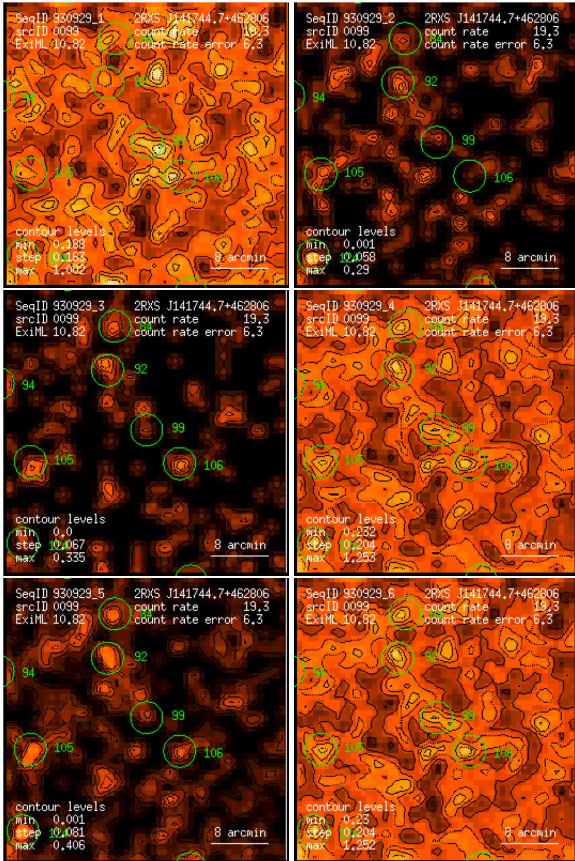
Figure 99: RASS 930929: detection 0099: band rate images, Gaussian filter: (1) PSPC channels 11 – 41, (2) 52 – 90, (3) 91 – 201, (4) 11 – 235, (5) 52 – 201, (6) 11 – 201. Broad band rates in counts/ks. Band rate contour levels in counts/ks/arcmin 2 .
