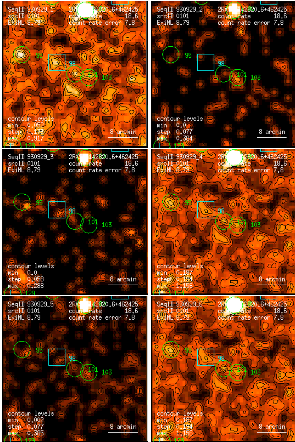
Figure 101: RASS 930929: detection 0101: band rate images, Gaussian filter: (1) PSPC channels 11 – 41, (2) 52 – 90, (3) 91 – 201, (4) 11 – 235, (5) 52 – 201, (6) 11 – 201. Broad band rates in counts/ks. Band rate contour levels in counts/ks/arcmin 2 .
