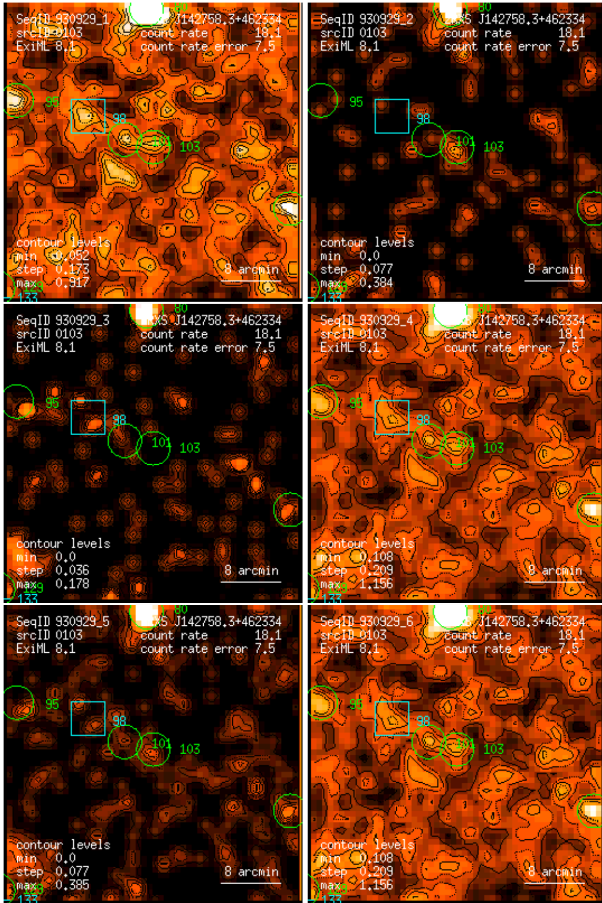
Figure 103: RASS 930929: detection 0103: band rate images, Gaussian filter: (1) PSPC channels 11 – 41, (2) 52 – 90, (3) 91 – 201, (4) 11 – 235, (5) 52 – 201, (6) 11 – 201. Broad band rates in counts/ks. Band rate contour levels in counts/ks/arcmin 2 .
