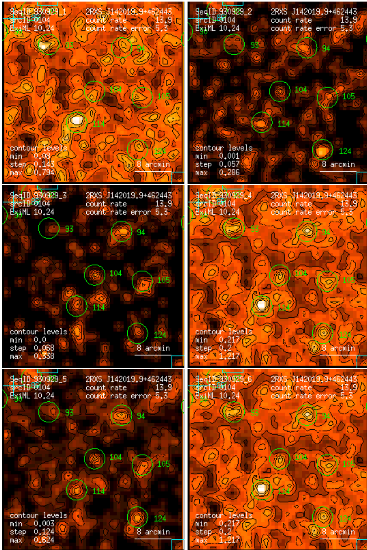
Figure 104: RASS 930929: detection 0104: band rate images, Gaussian filter: (1) PSPC channels 11 – 41, (2) 52 – 90, (3) 91 – 201, (4) 11 – 235, (5) 52 – 201, (6) 11 – 201. Broad band rates in counts/ks. Band rate contour levels in counts/ks/arcmin 2 .
