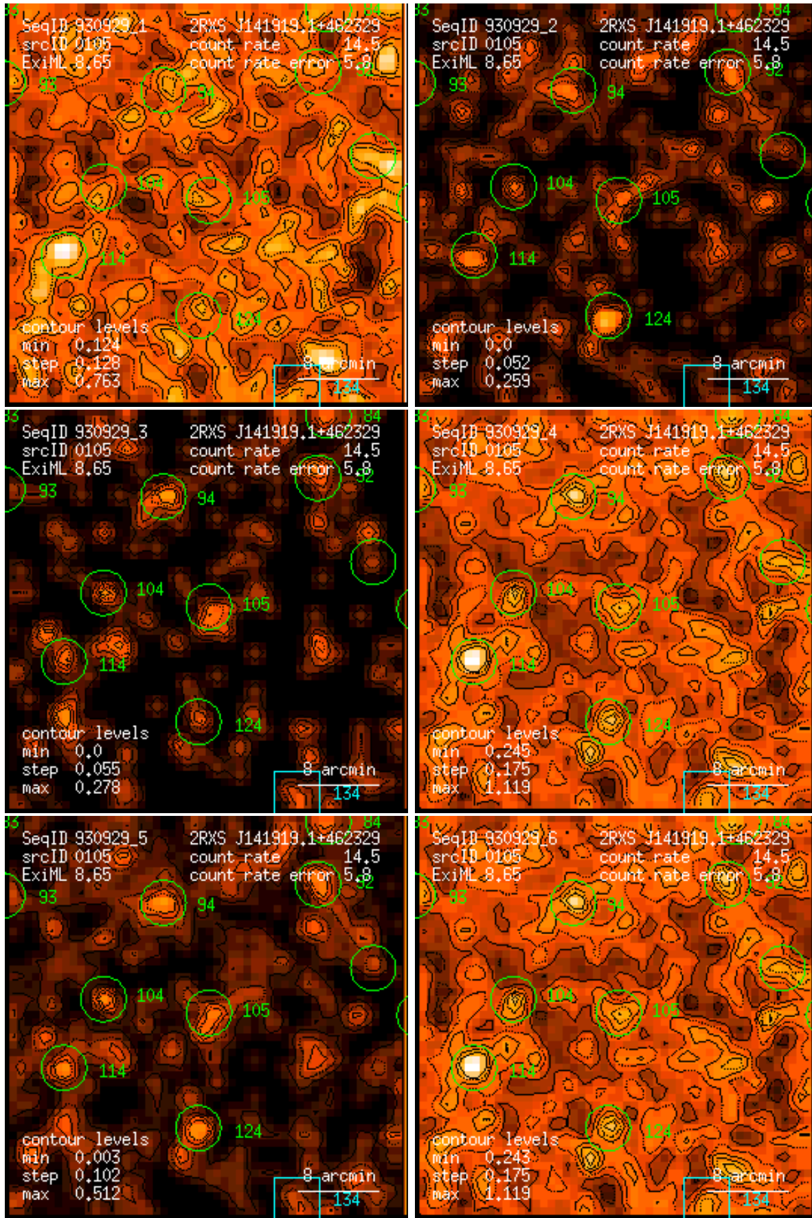
Figure 105: RASS 930929: detection 0105: band rate images, Gaussian filter: (1) PSPC channels 11 – 41, (2) 52 – 90, (3) 91 – 201, (4) 11 – 235, (5) 52 – 201, (6) 11 – 201. Broad band rates in counts/ks. Band rate contour levels in counts/ks/arcmin 2 .
