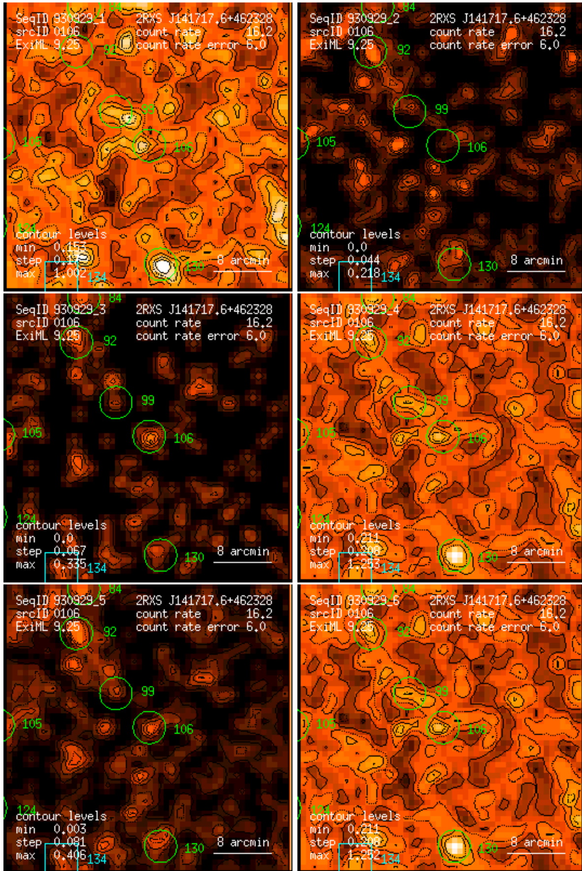
Figure 106: RASS 930929: detection 0106: band rate images, Gaussian filter: (1) PSPC channels 11 – 41, (2) 52 – 90, (3) 91 – 201, (4) 11 – 235, (5) 52 – 201, (6) 11 – 201. Broad band rates in counts/ks. Band rate contour levels in counts/ks/arcmin 2 .
