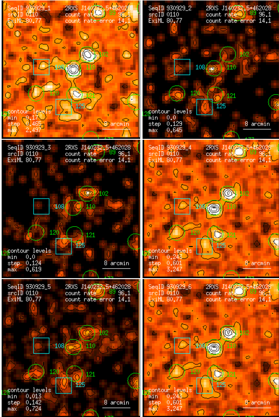
Figure 110: RASS 930929: detection 0110: band rate images, Gaussian filter: (1) PSPC channels 11 – 41, (2) 52 – 90, (3) 91 – 201, (4) 11 – 235, (5) 52 – 201, (6) 11 – 201. Broad band rates in counts/ks. Band rate contour levels in counts/ks/arcmin 2 .
