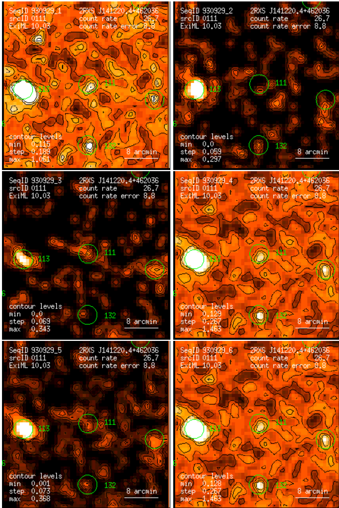
Figure 111: RASS 930929: detection 0111: band rate images, Gaussian filter: (1) PSPC channels 11 – 41, (2) 52 – 90, (3) 91 – 201, (4) 11 – 235, (5) 52 – 201, (6) 11 – 201. Broad band rates in counts/ks. Band rate contour levels in counts/ks/arcmin 2 .
