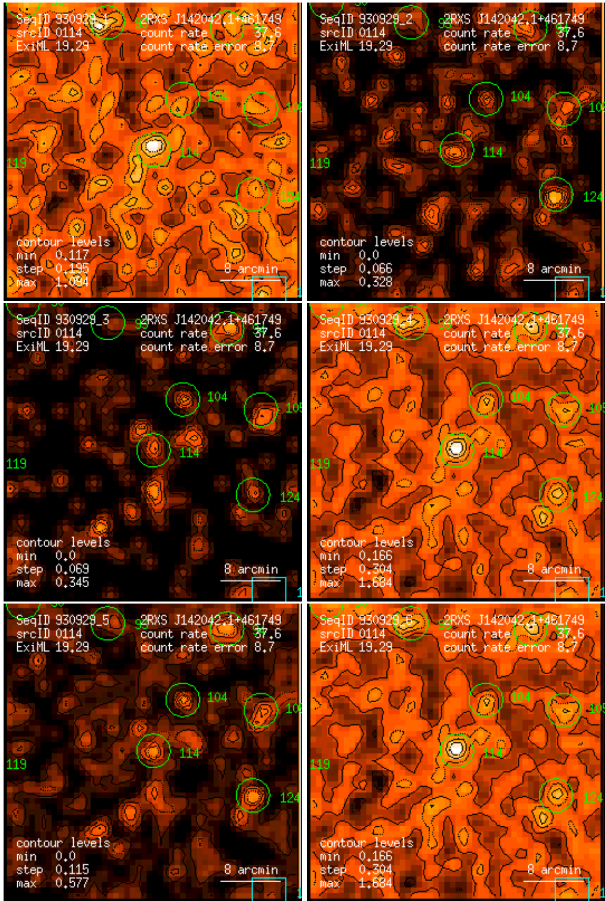
Figure 114: RASS 930929: detection 0114: band rate images, Gaussian filter: (1) PSPC channels 11 – 41, (2) 52 – 90, (3) 91 – 201, (4) 11 – 235, (5) 52 – 201, (6) 11 – 201. Broad band rates in counts/ks. Band rate contour levels in counts/ks/arcmin 2 .
