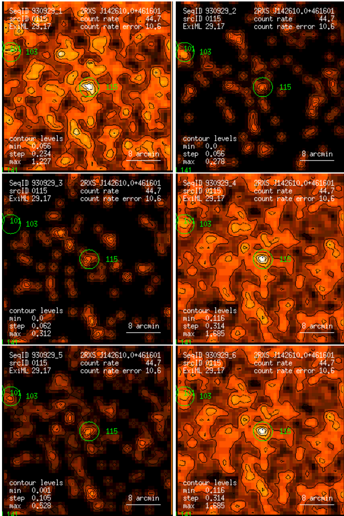
Figure 115: RASS 930929: detection 0115: band rate images, Gaussian filter: (1) PSPC channels 11 – 41, (2) 52 – 90, (3) 91 – 201, (4) 11 – 235, (5) 52 – 201, (6) 11 – 201. Broad band rates in counts/ks. Band rate contour levels in counts/ks/arcmin 2 .
