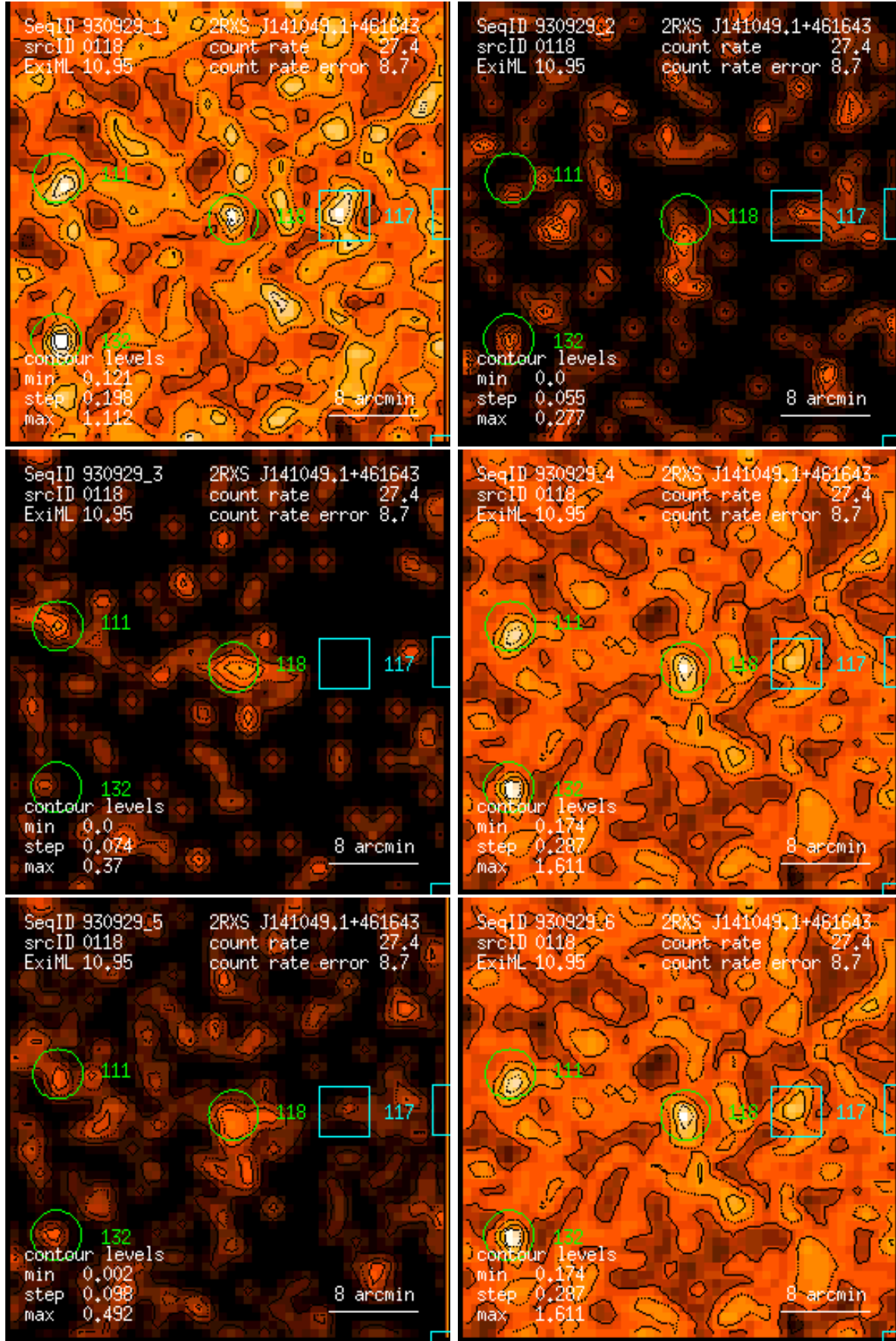
Figure 118: RASS 930929: detection 0118: band rate images, Gaussian filter: (1) PSPC channels 11 – 41, (2) 52 – 90, (3) 91 – 201, (4) 11 – 235, (5) 52 – 201, (6) 11 – 201. Broad band rates in counts/ks. Band rate contour levels in counts/ks/arcmin 2 .
