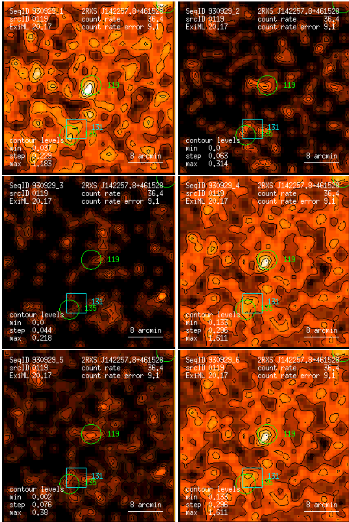
Figure 119: RASS 930929: detection 0119: band rate images, Gaussian filter: (1) PSPC channels 11 – 41, (2) 52 – 90, (3) 91 – 201, (4) 11 – 235, (5) 52 – 201, (6) 11 – 201. Broad band rates in counts/ks. Band rate contour levels in counts/ks/arcmin 2 .
