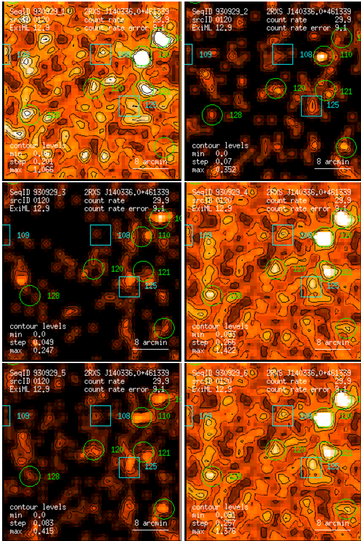
Figure 120: RASS 930929: detection 0120: band rate images, Gaussian filter: (1) PSPC channels 11 – 41, (2) 52 – 90, (3) 91 – 201, (4) 11 – 235, (5) 52 – 201, (6) 11 – 201. Broad band rates in counts/ks. Band rate contour levels in counts/ks/arcmin 2 .
