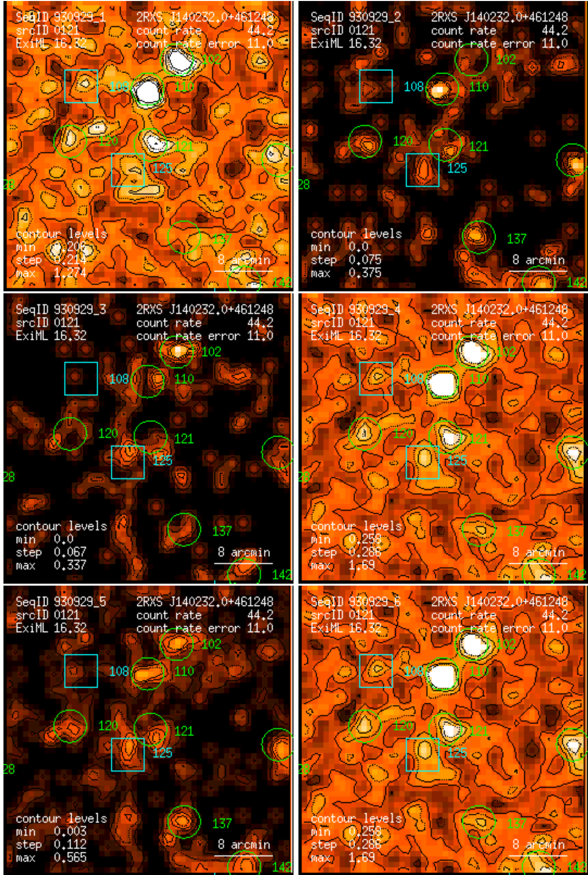
Figure 121: RASS 930929: detection 0121: band rate images, Gaussian filter: (1) PSPC channels 11 – 41, (2) 52 – 90, (3) 91 – 201, (4) 11 – 235, (5) 52 – 201, (6) 11 – 201. Broad band rates in counts/ks. Band rate contour levels in counts/ks/arcmin 2 .
