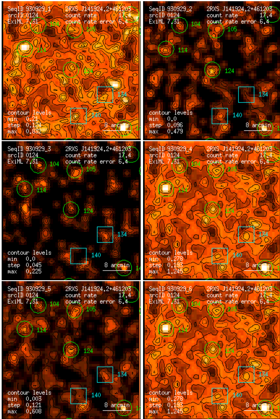
Figure 124: RASS 930929: detection 0124: band rate images, Gaussian filter: (1) PSPC channels 11 – 41, (2) 52 – 90, (3) 91 – 201, (4) 11 – 235, (5) 52 – 201, (6) 11 – 201. Broad band rates in counts/ks. Band rate contour levels in counts/ks/arcmin 2 .
