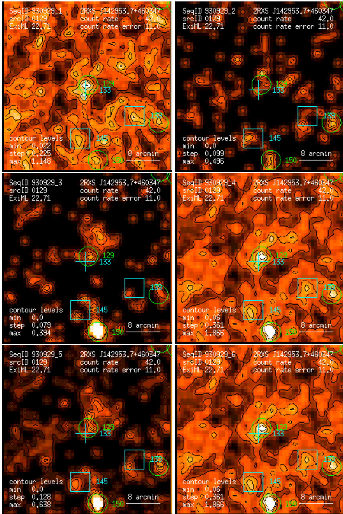
Figure 129: RASS 930929: detection 0129: band rate images, Gaussian filter: (1) PSPC channels 11 – 41, (2) 52 – 90, (3) 91 – 201, (4) 11 – 235, (5) 52 – 201, (6) 11 – 201. Broad band rates in counts/ks. Band rate contour levels in counts/ks/arcmin 2 .
