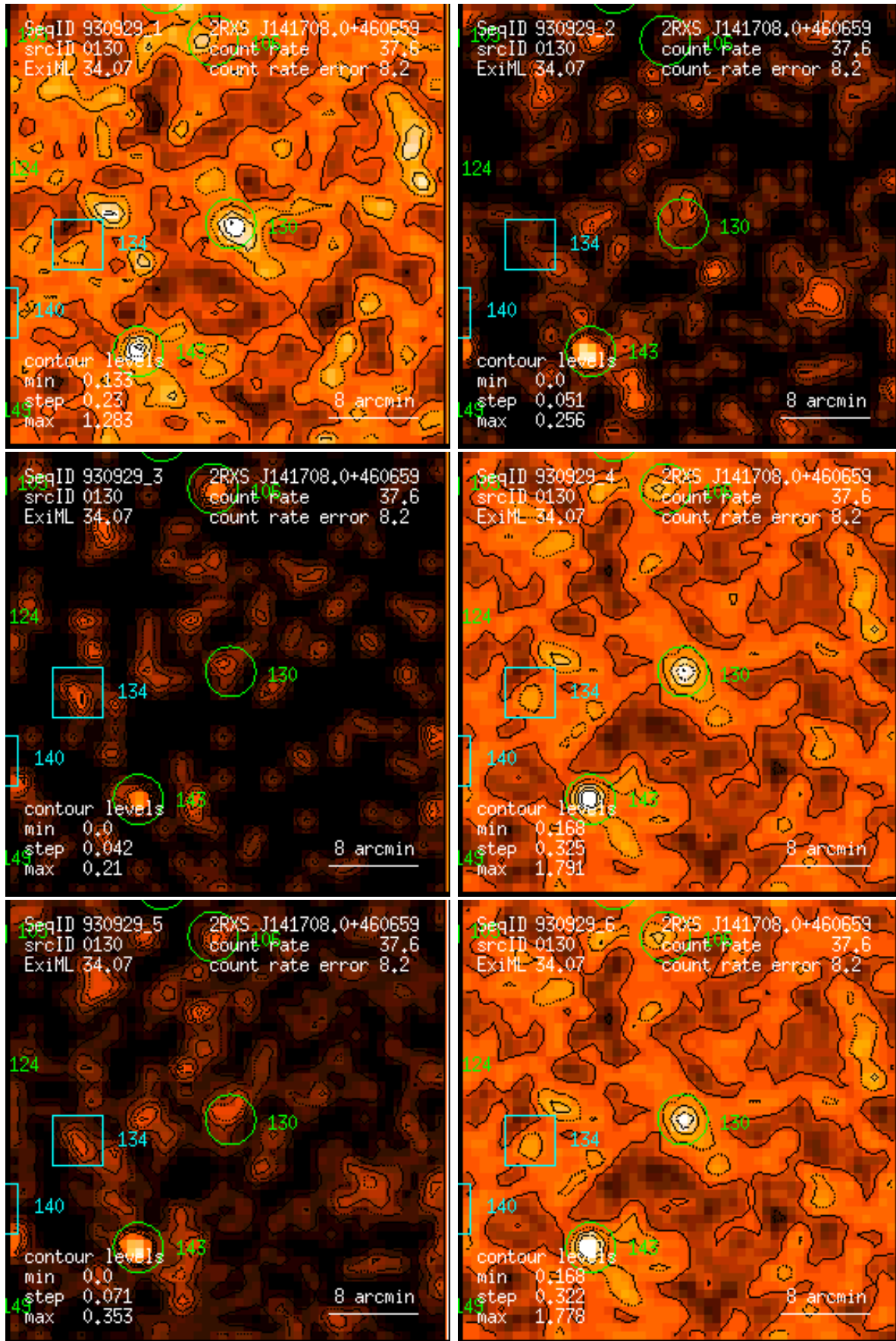
Figure 130: RASS 930929: detection 0130: band rate images, Gaussian filter: (1) PSPC channels 11 – 41, (2) 52 – 90, (3) 91 – 201, (4) 11 – 235, (5) 52 – 201, (6) 11 – 201. Broad band rates in counts/ks. Band rate contour levels in counts/ks/arcmin 2 .
