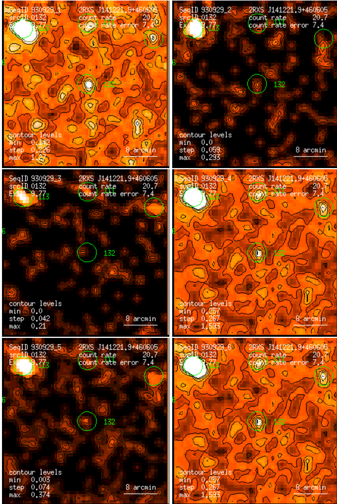
Figure 132: RASS 930929: detection 0132: band rate images, Gaussian filter: (1) PSPC channels 11 – 41, (2) 52 – 90, (3) 91 – 201, (4) 11 – 235, (5) 52 – 201, (6) 11 – 201. Broad band rates in counts/ks. Band rate contour levels in counts/ks/arcmin 2 .
