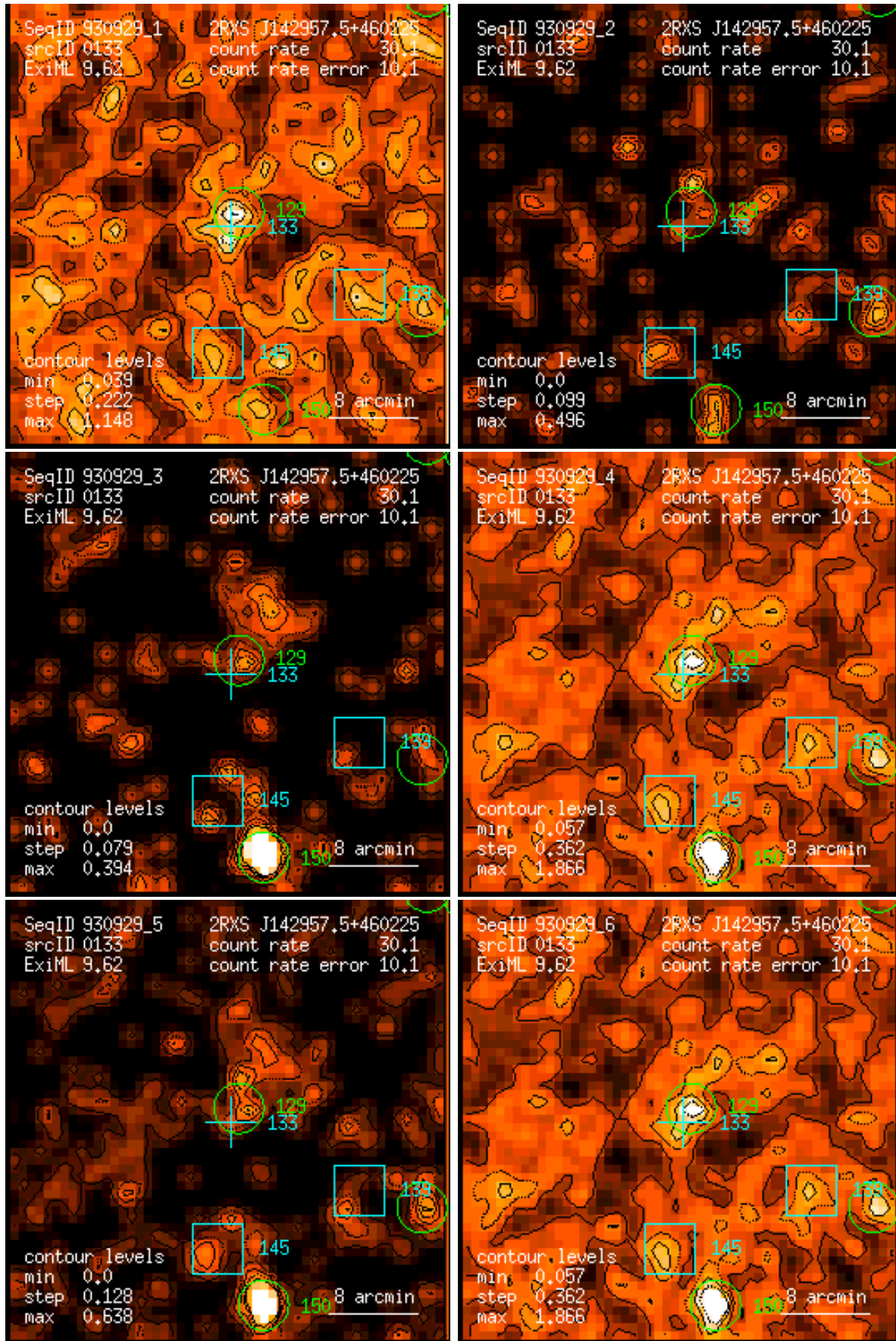
Figure 133: RASS 930929: detection 0133: band rate images, Gaussian filter: (1) PSPC channels 11 – 41, (2) 52 – 90, (3) 91 – 201, (4) 11 – 235, (5) 52 – 201, (6) 11 – 201. Broad band rates in counts/ks. Band rate contour levels in counts/ks/arcmin 2 .
