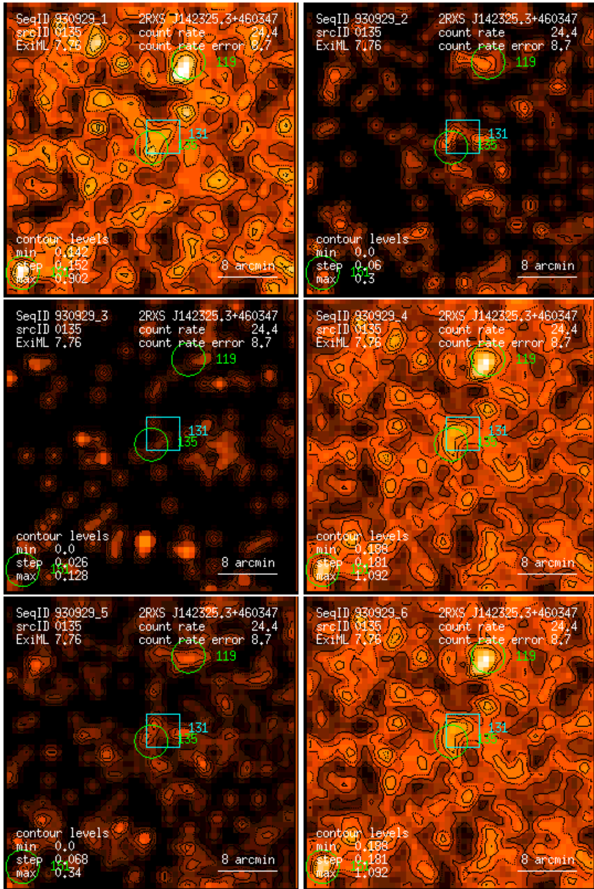
Figure 135: RASS 930929: detection 0135: band rate images, Gaussian filter: (1) PSPC channels 11 – 41, (2) 52 – 90, (3) 91 – 201, (4) 11 – 235, (5) 52 – 201, (6) 11 – 201. Broad band rates in counts/ks. Band rate contour levels in counts/ks/arcmin 2 .
