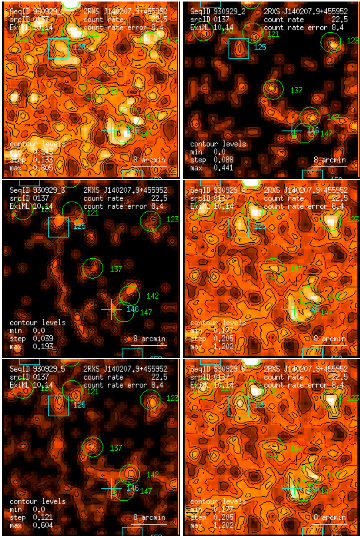
Figure 137: RASS 930929: detection 0137: band rate images, Gaussian filter: (1) PSPC channels 11 – 41, (2) 52 – 90, (3) 91 – 201, (4) 11 – 235, (5) 52 – 201, (6) 11 – 201. Broad band rates in counts/ks. Band rate contour levels in counts/ks/arcmin 2 .
