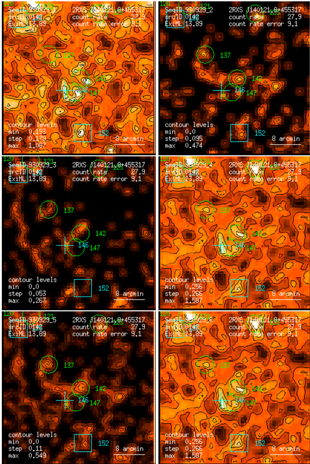
Figure 142: RASS 930929: detection 0142: band rate images, Gaussian filter: (1) PSPC channels 11 – 41, (2) 52 – 90, (3) 91 – 201, (4) 11 – 235, (5) 52 – 201, (6) 11 – 201. Broad band rates in counts/ks. Band rate contour levels in counts/ks/arcmin 2 .
