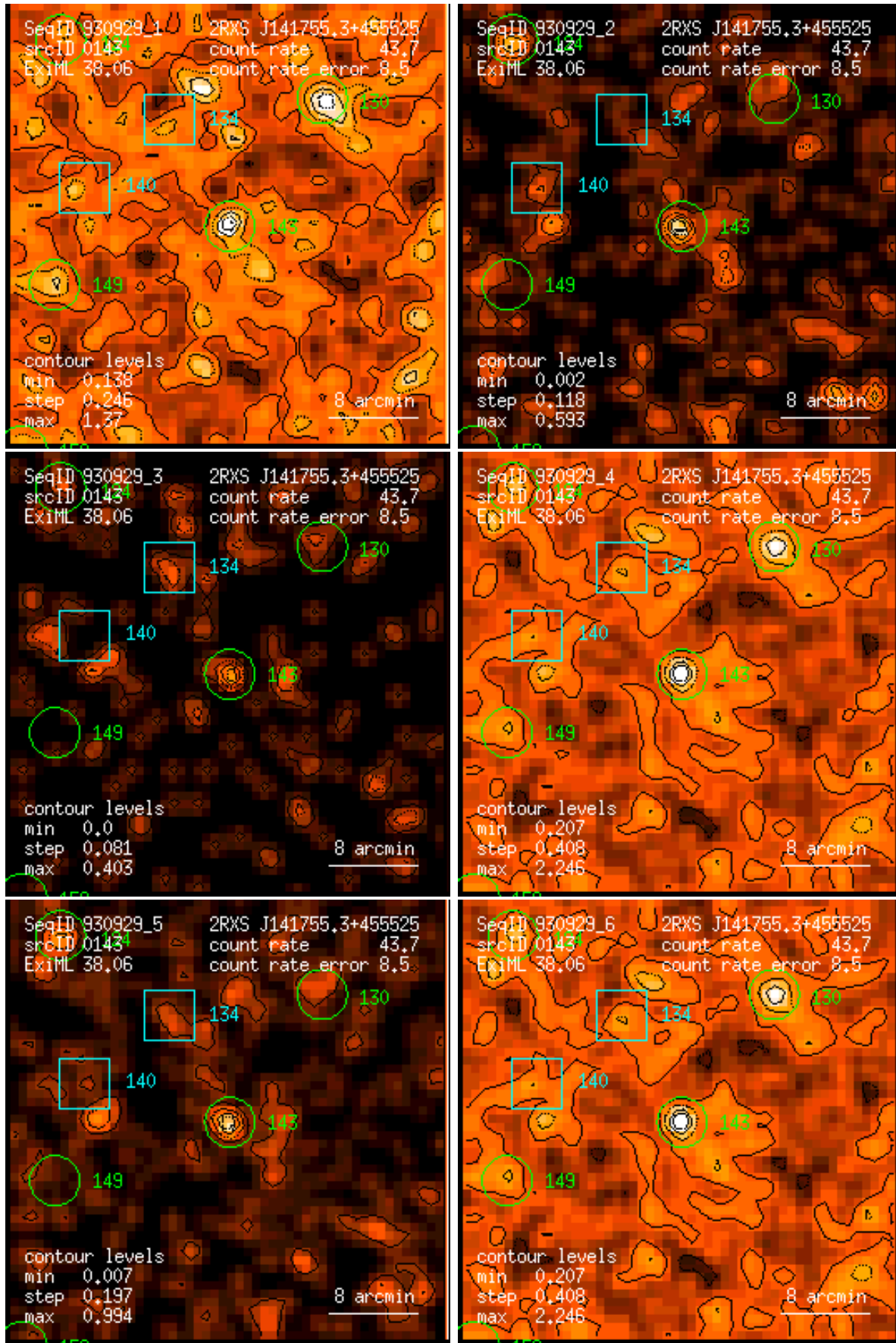
Figure 143: RASS 930929: detection 0143: band rate images, Gaussian filter: (1) PSPC channels 11 – 41, (2) 52 – 90, (3) 91 – 201, (4) 11 – 235, (5) 52 – 201, (6) 11 – 201. Broad band rates in counts/ks. Band rate contour levels in counts/ks/arcmin 2 .
