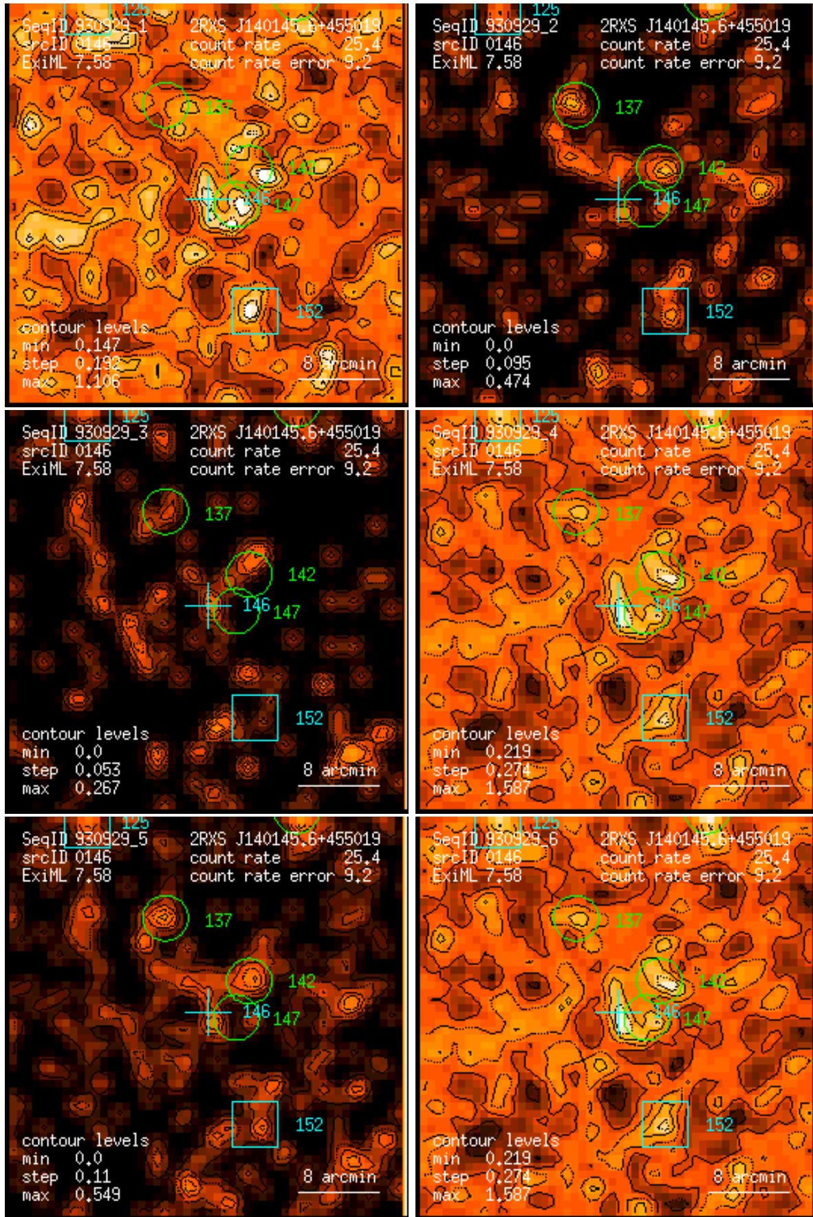
Figure 146: RASS 930929: detection 0146: band rate images, Gaussian filter: (1) PSPC channels 11 – 41, (2) 52 – 90, (3) 91 – 201, (4) 11 – 235, (5) 52 – 201, (6) 11 – 201. Broad band rates in counts/ks. Band rate contour levels in counts/ks/arcmin 2 .
