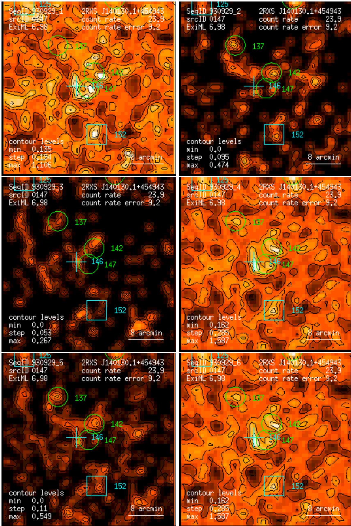
Figure 147: RASS 930929: detection 0147: band rate images, Gaussian filter: (1) PSPC channels 11 – 41, (2) 52 – 90, (3) 91 – 201, (4) 11 – 235, (5) 52 – 201, (6) 11 – 201. Broad band rates in counts/ks. Band rate contour levels in counts/ks/arcmin 2 .
