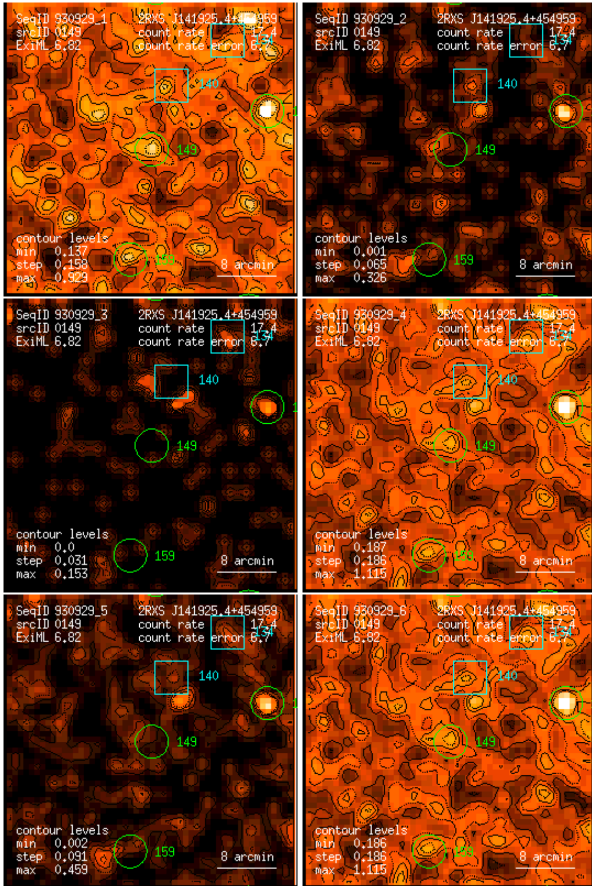
Figure 149: RASS 930929: detection 0149: band rate images, Gaussian filter: (1) PSPC channels 11 – 41, (2) 52 – 90, (3) 91 – 201, (4) 11 – 235, (5) 52 – 201, (6) 11 – 201. Broad band rates in counts/ks. Band rate contour levels in counts/ks/arcmin 2 .
