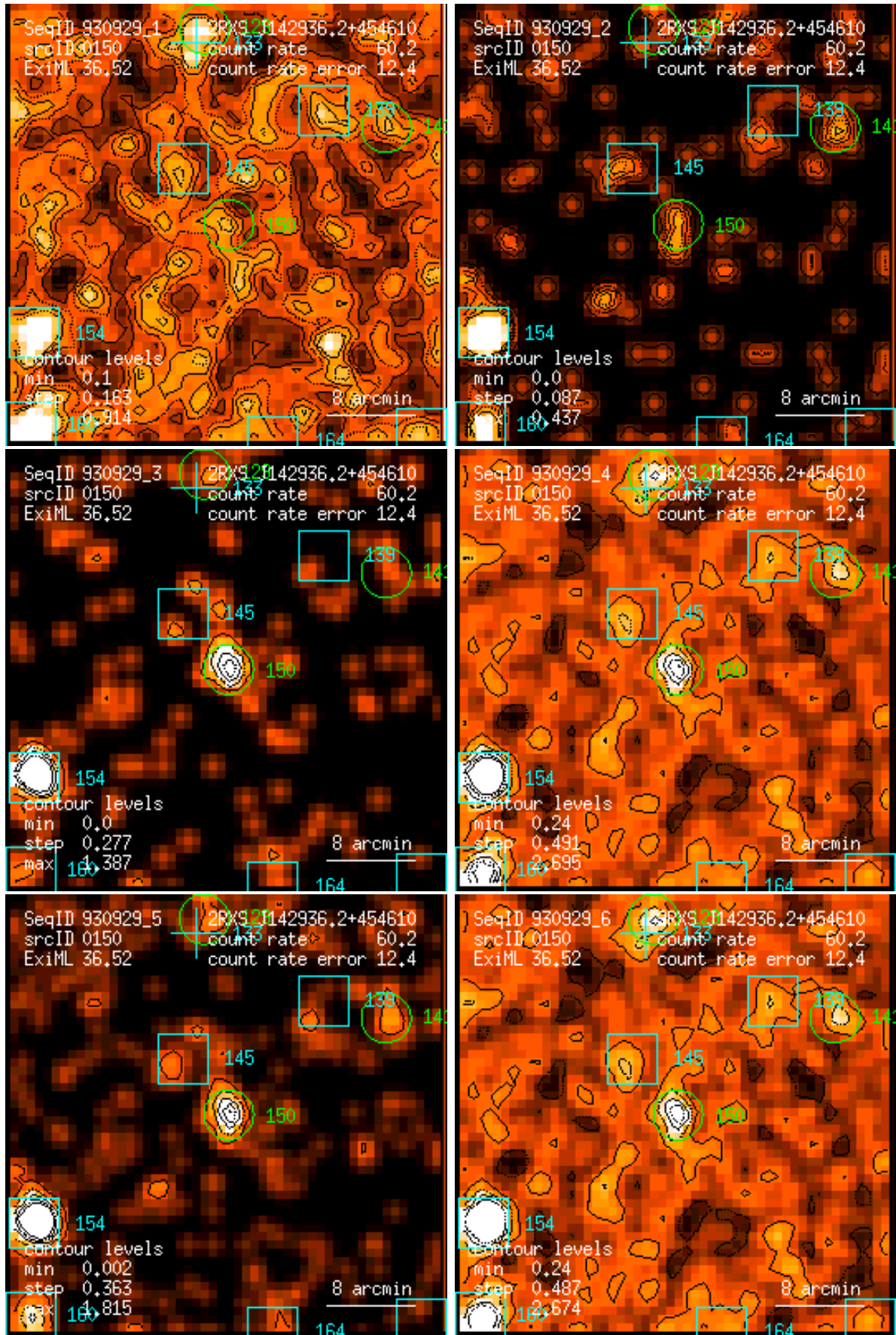
Figure 150: RASS 930929: detection 0150: band rate images, Gaussian filter: (1) PSPC channels 11 – 41, (2) 52 – 90, (3) 91 – 201, (4) 11 – 235, (5) 52 – 201, (6) 11 – 201. Broad band rates in counts/ks. Band rate contour levels in counts/ks/arcmin 2 .
