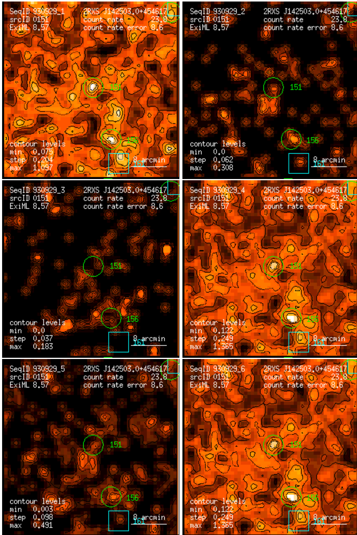
Figure 151: RASS 930929: detection 0151: band rate images, Gaussian filter: (1) PSPC channels 11 – 41, (2) 52 – 90, (3) 91 – 201, (4) 11 – 235, (5) 52 – 201, (6) 11 – 201. Broad band rates in counts/ks. Band rate contour levels in counts/ks/arcmin 2 .
