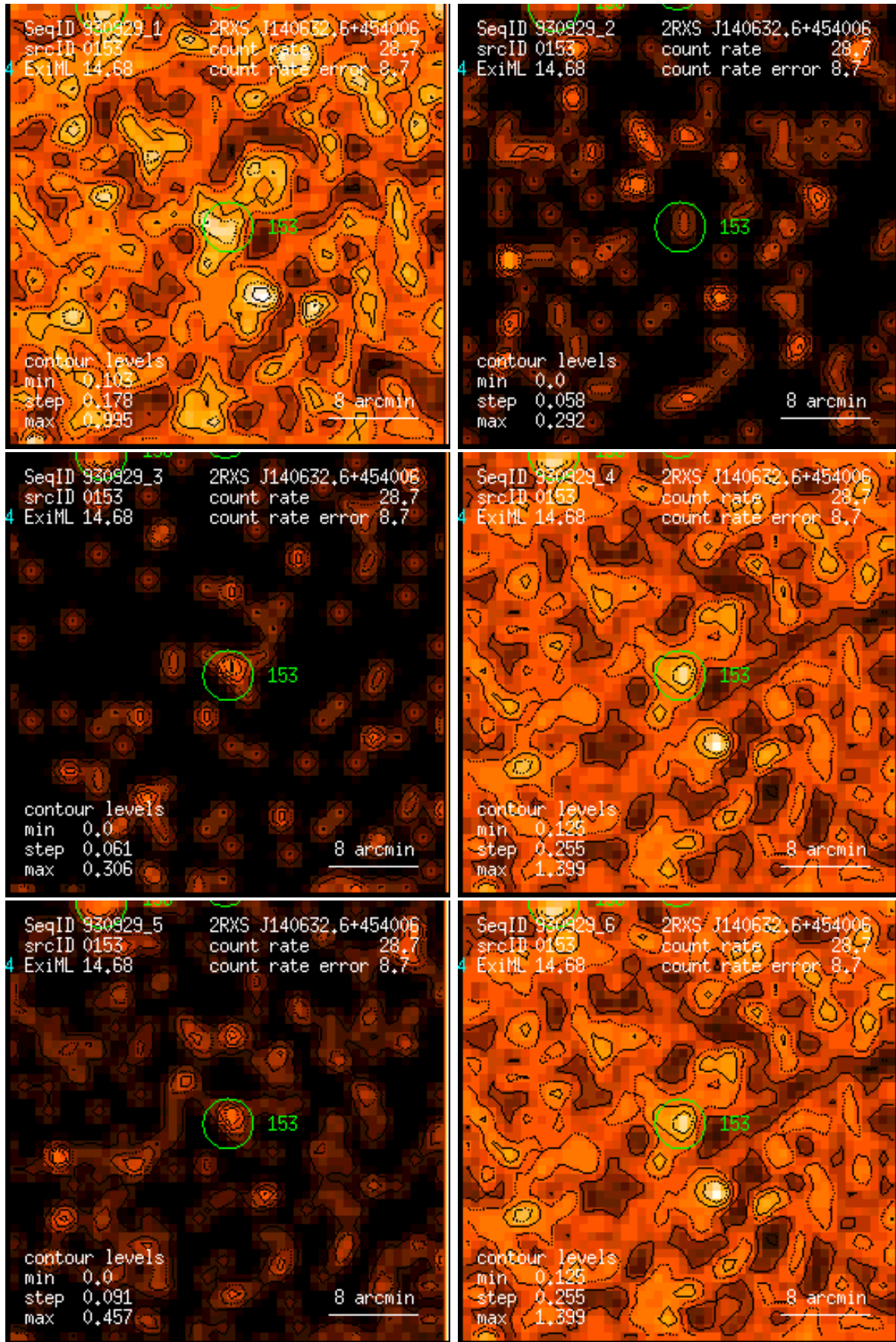
Figure 153: RASS 930929: detection 0153: band rate images, Gaussian filter: (1) PSPC channels 11 – 41, (2) 52 – 90, (3) 91 – 201, (4) 11 – 235, (5) 52 – 201, (6) 11 – 201. Broad band rates in counts/ks. Band rate contour levels in counts/ks/arcmin 2 .
