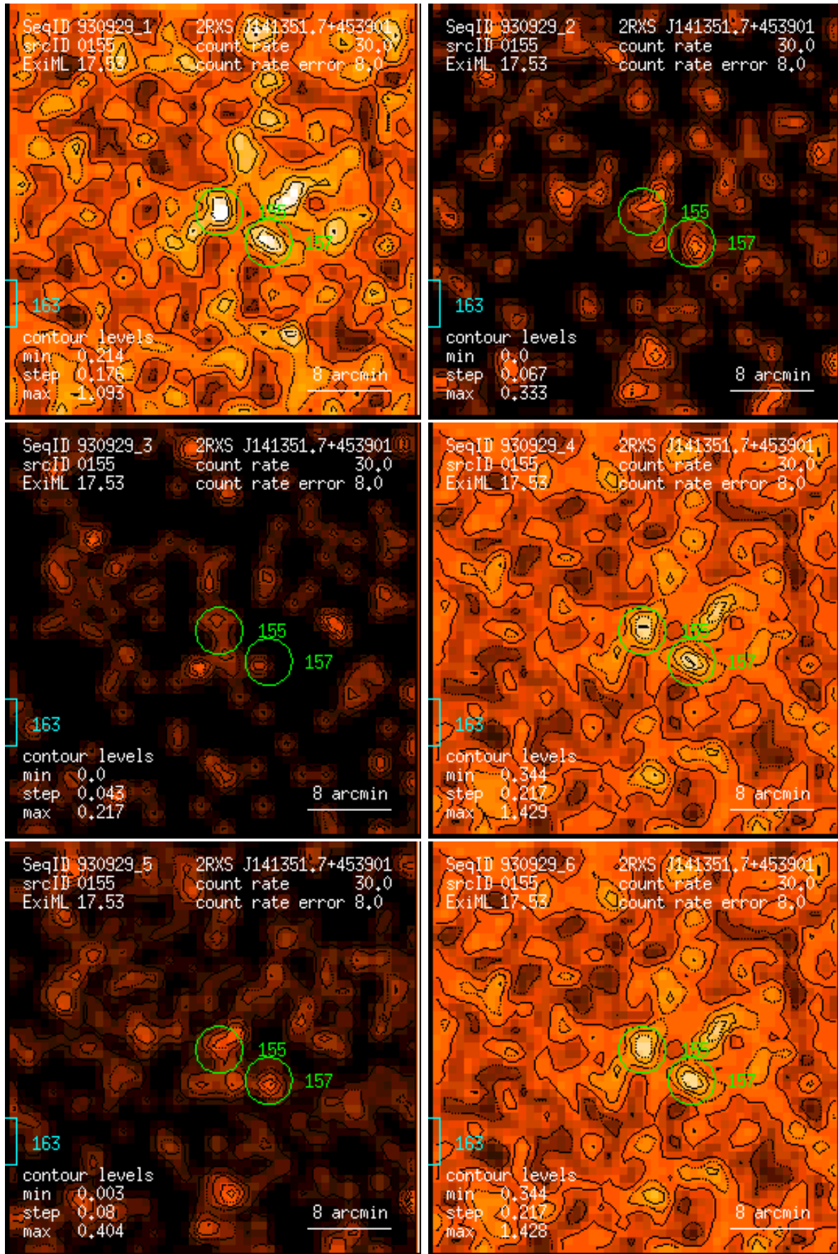
Figure 155: RASS 930929: detection 0155: band rate images, Gaussian filter: (1) PSPC channels 11 – 41, (2) 52 – 90, (3) 91 – 201, (4) 11 – 235, (5) 52 – 201, (6) 11 – 201. Broad band rates in counts/ks. Band rate contour levels in counts/ks/arcmin 2 .
