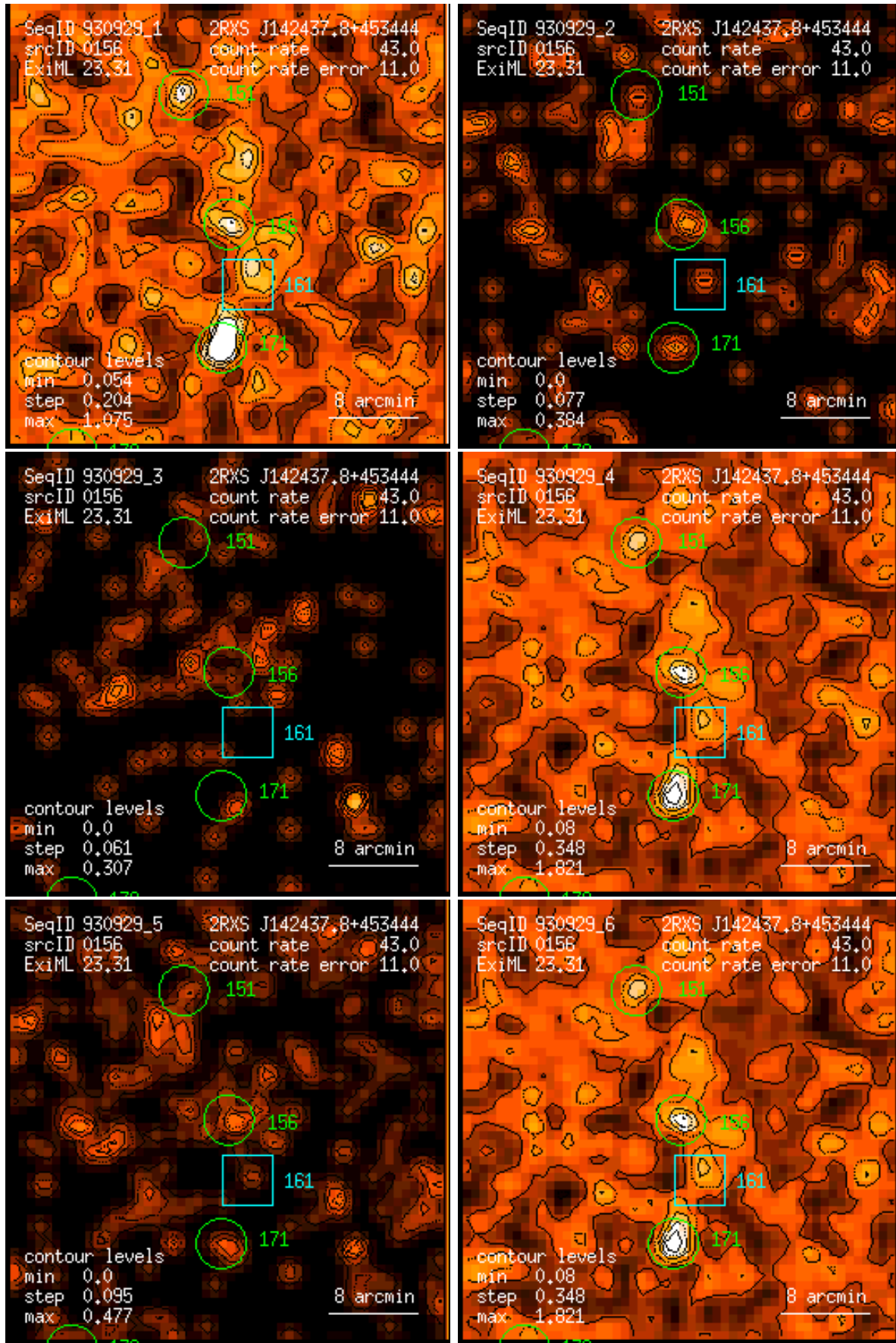
Figure 156: RASS 930929: detection 0156: band rate images, Gaussian filter: (1) PSPC channels 11 – 41, (2) 52 – 90, (3) 91 – 201, (4) 11 – 235, (5) 52 – 201, (6) 11 – 201. Broad band rates in counts/ks. Band rate contour levels in counts/ks/arcmin 2 .
